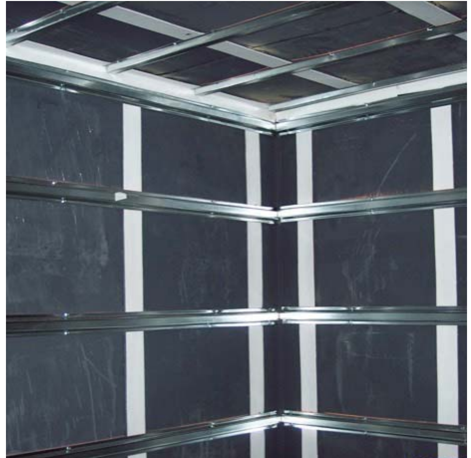
Vault Panels with Vapor Barrier and Magnetic Shielding on Interior. Vault is ready for drywall finish and light fixtures
