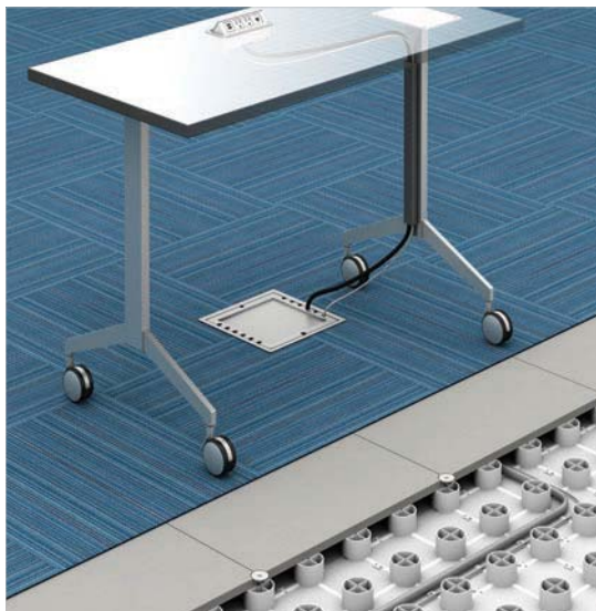
Access power and data virtually anywhere within the system grid. Modular floor elements rise 2" above existing subfloor.
